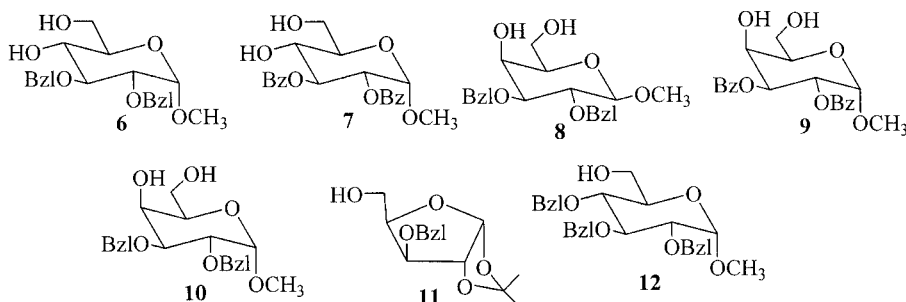
Figure 3. Cyclic mono- and dihydroxy sugar derivatives as glycosyl acceptors.
