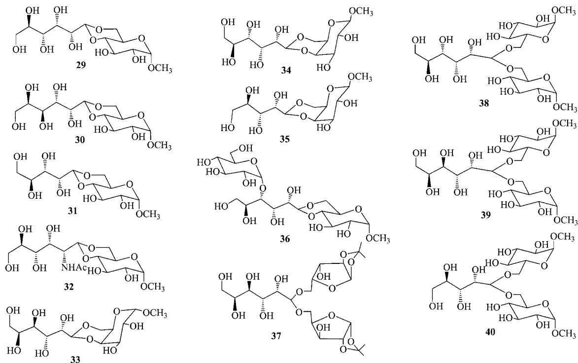
Figure 6. Deprotected di- and trisaccharides containing acetal linkages.
