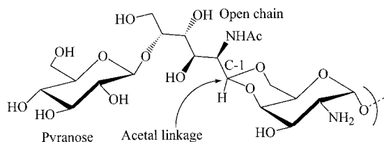
Figure 1. A new type of glycosyl linkage found in the cell wall of Proteus bacteria.
