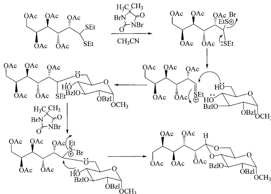
Scheme 2. Plausible mechanism for the formation of acyclic glycosylidene glycoside.
