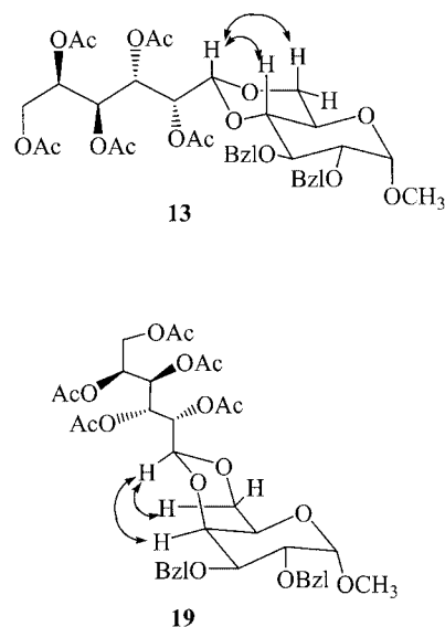
Figure 7. NOE enhancement observed between acyclic H-1 and H-4 and H-6 of cyclic sugars.
