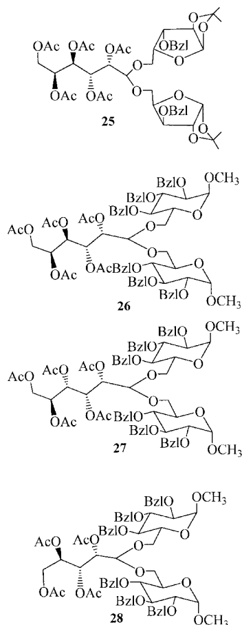
Figure 5. Synthesized acetal-linked acyclic-cyclic sugar trisaccharides.
