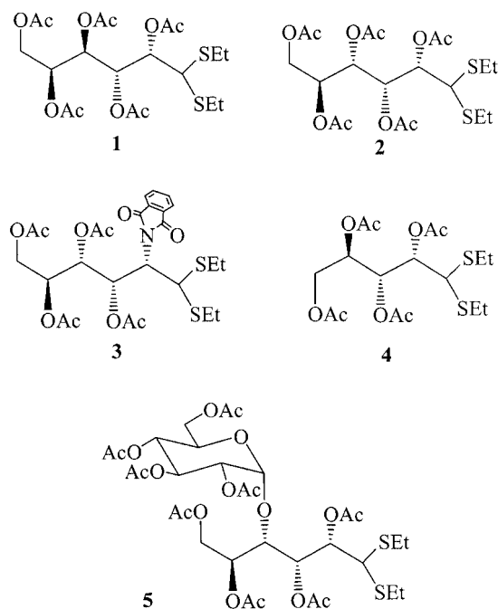
Figure 2. Acyclic glycosyl dithioacetals as glycosyl donors.
