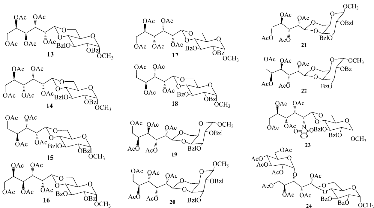
Figure 4. Synthesized acetal-linked acyclic-cyclic sugar disaccharides.
